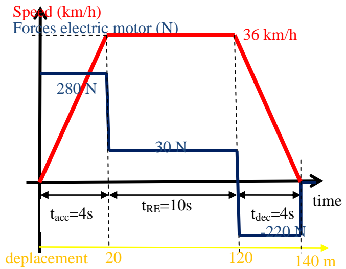
Fig 2 : speed and force motor resultant according to time for a mass M=100 kg, F_{Resistance}=30N .
