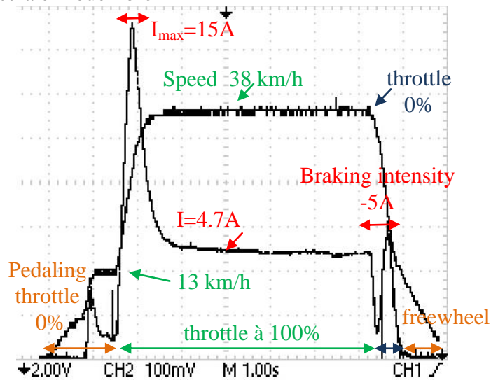
Fig 5 : speed and intensity battery according to time with no load (F R 23N, wheel mass 7kg)
